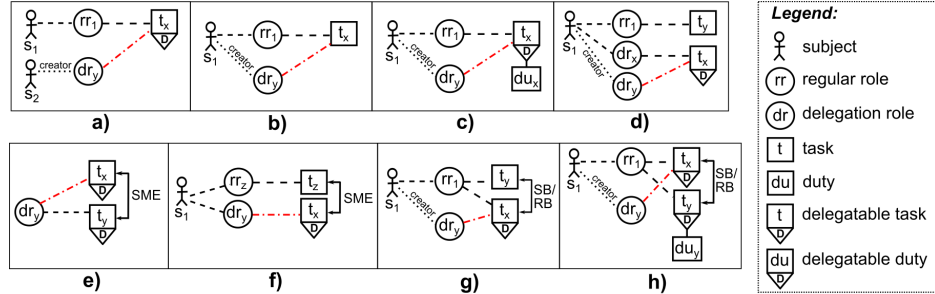
Fig. 2. Delegation conflicts
