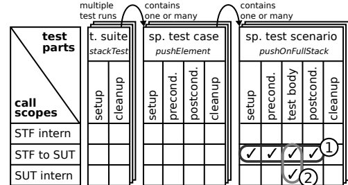
Figure 7: Example of option space for defining views on test-execution traces, by combining scenario-test parts and feature-call scopes
