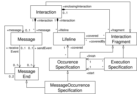
Figure 5: Selected elements of UML2 interaction models
