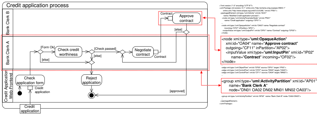
Figure 4: Example of an UML2 activity model and its XMI representation
